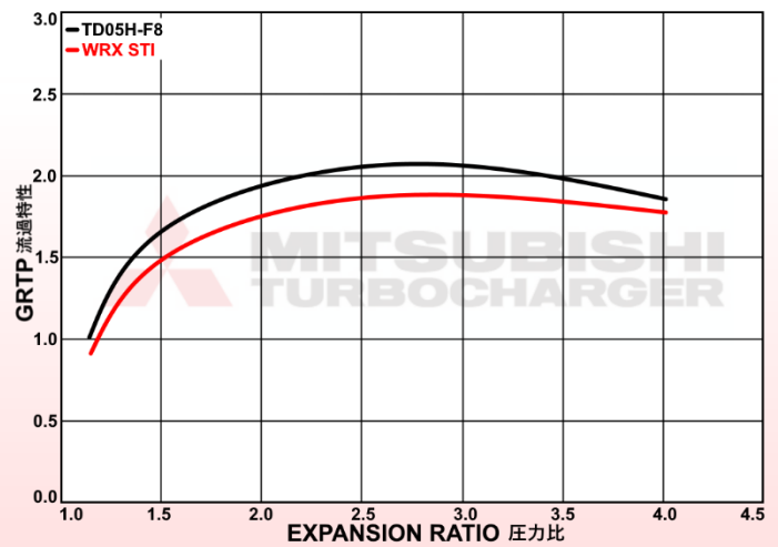
TURBINE MAP
