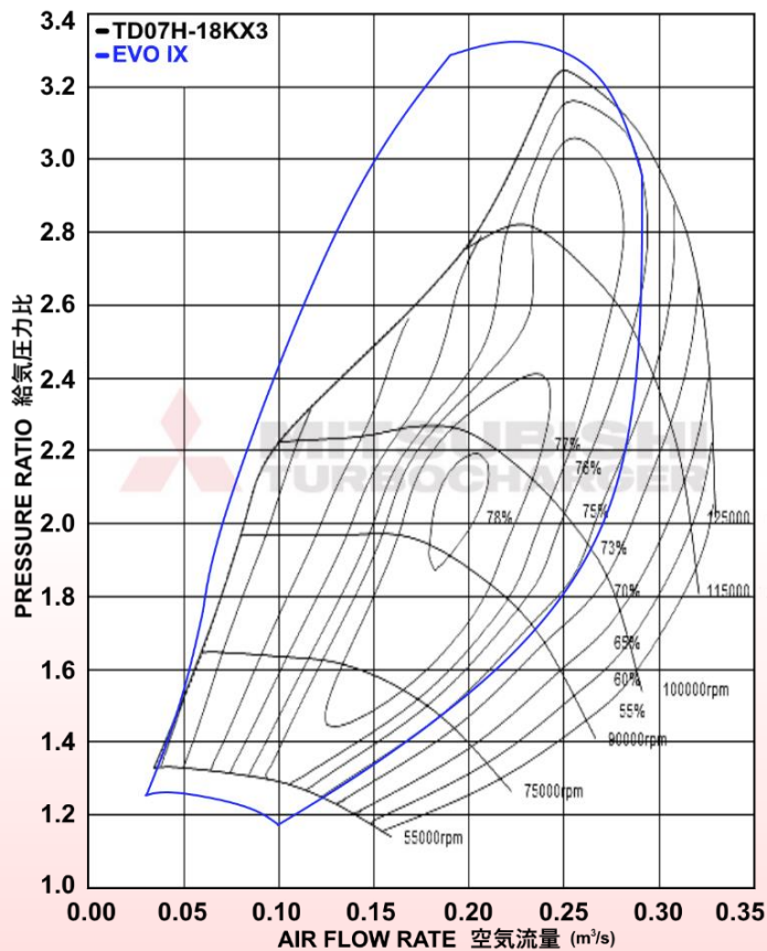
COMPRESSOR MAP
