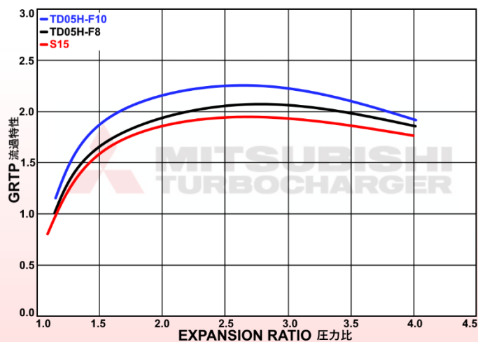
TURBINE MAP
