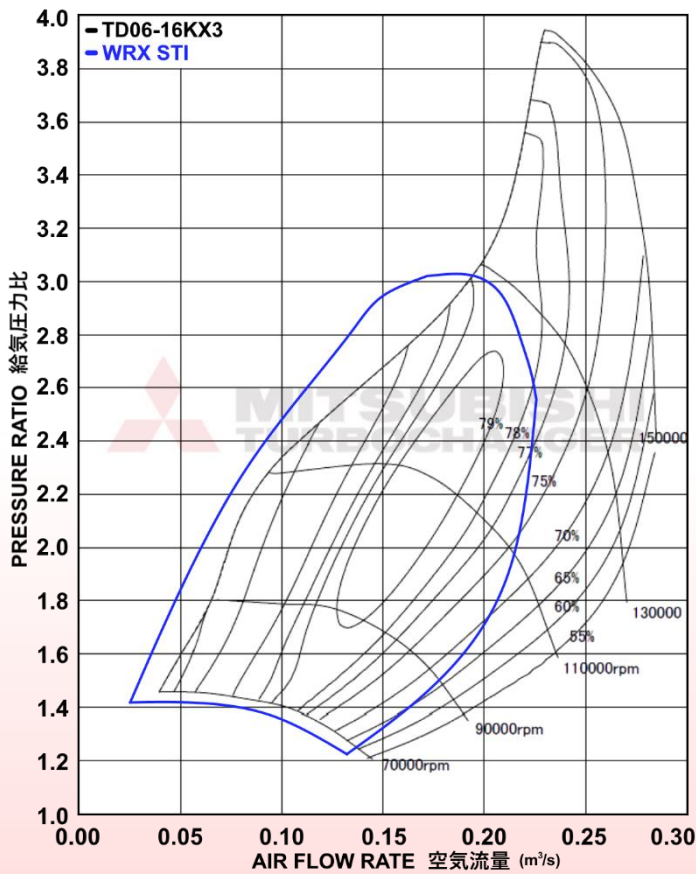
COMPRESSOR MAP
