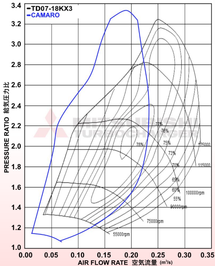
COMPRESSOR MAP
