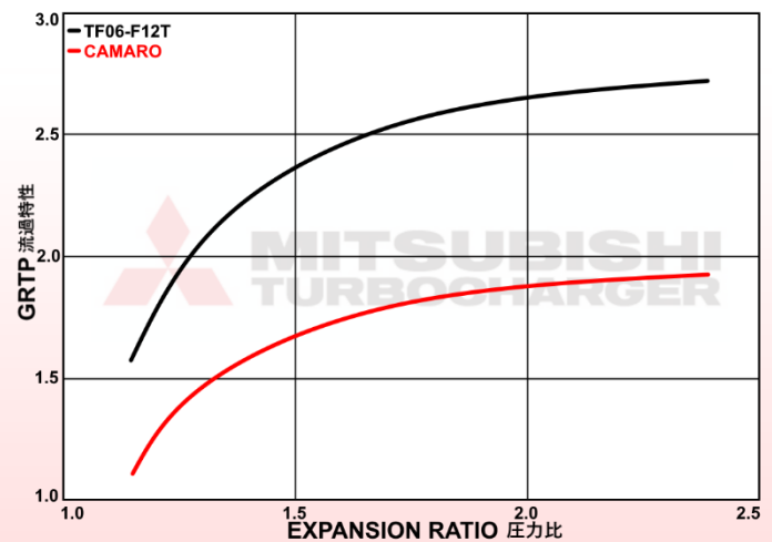
TURBINE MAP
