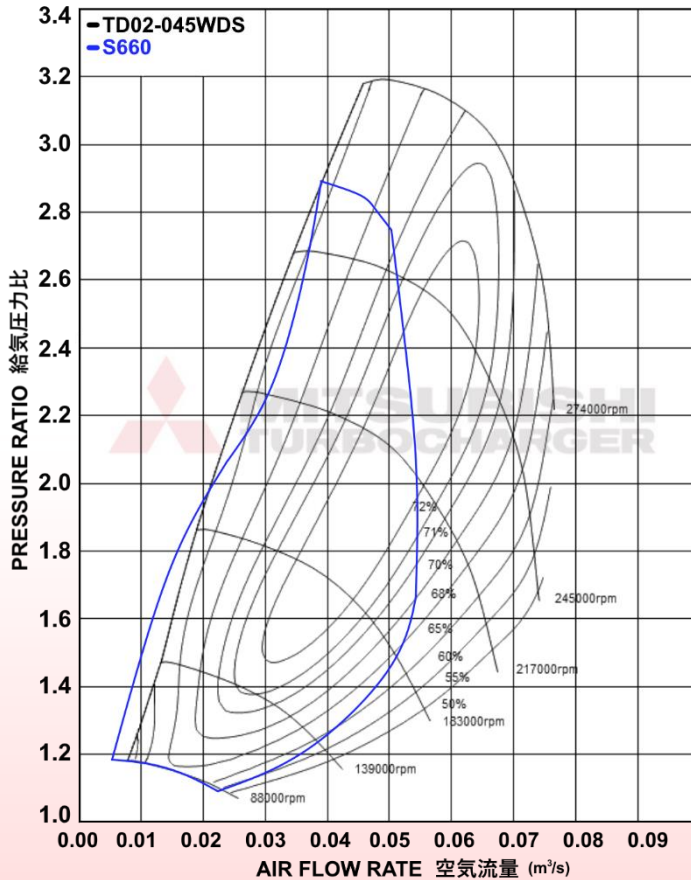
COMPRESSOR MAP
