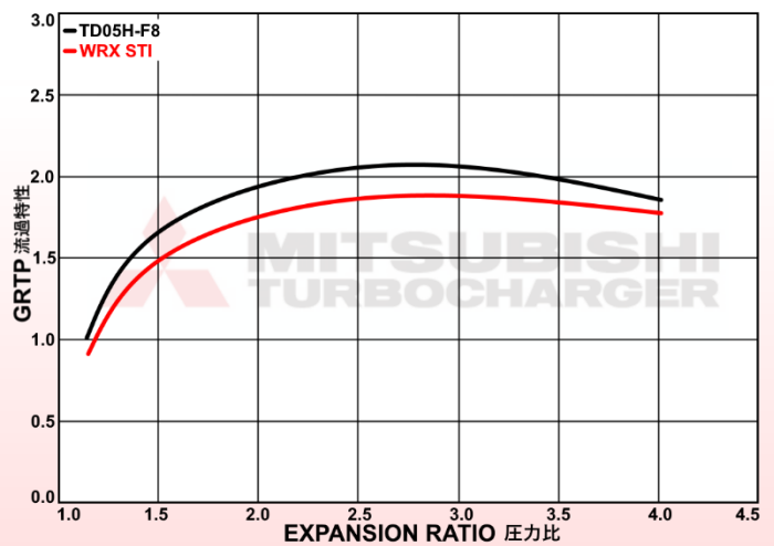
TURBINE MAP
