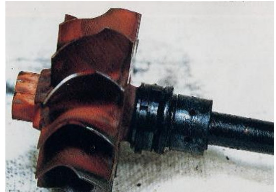
Turbine rotor with oil coking on the bearing
