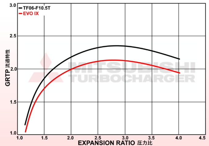
TURBINE MAP
