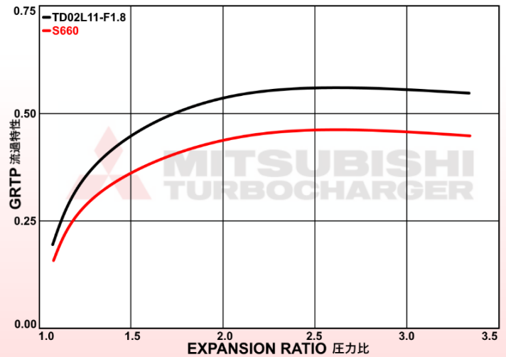
TURBINE MAP
