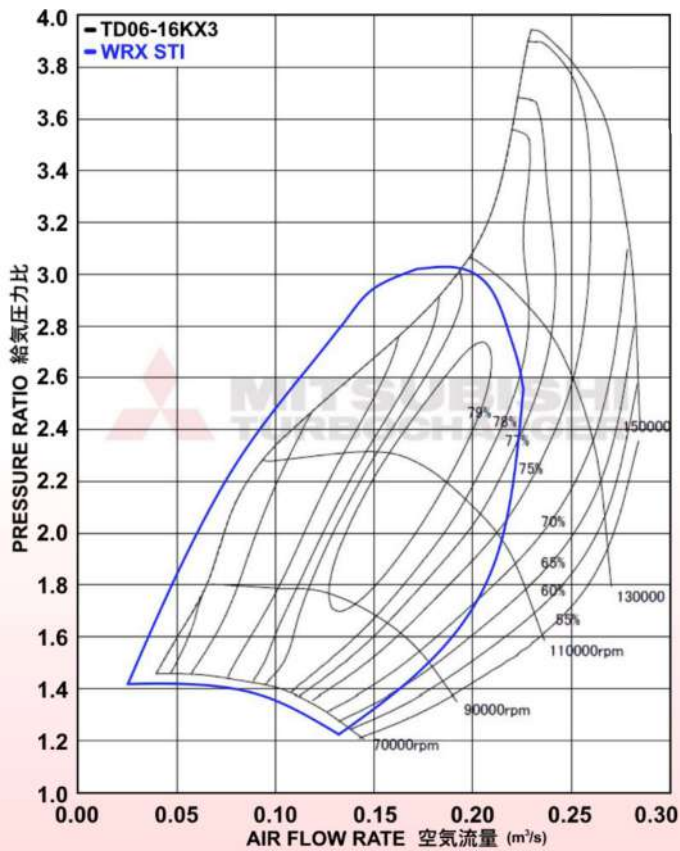
COMPRESSOR MAP
